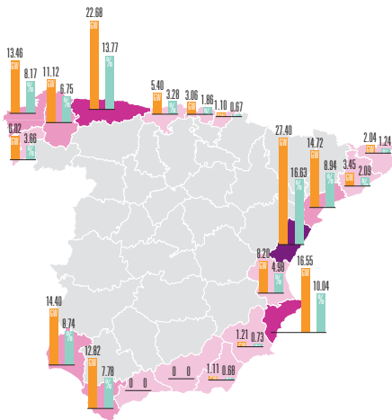
Division by provinces of capacity ceilings and electricity generation on the peninsula with this technology
