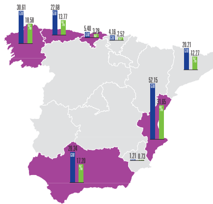
Division by Autonomous Communities of capacity ceilings and electricity generation on the peninsula with this technology
