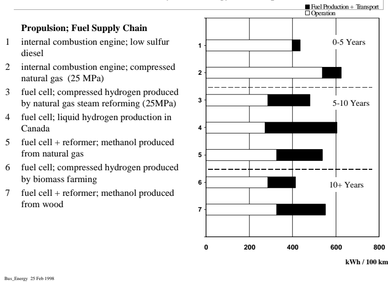
Fig. 6: Energy consumption of low floor city bus
